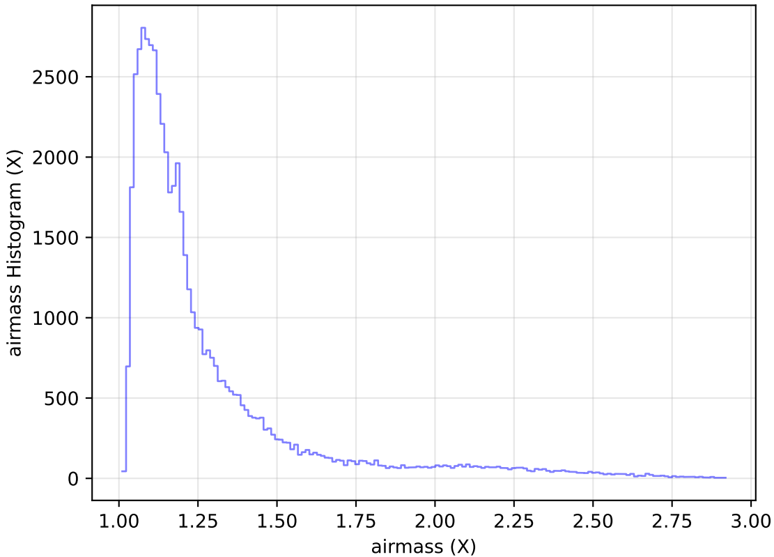
too_ignore_5_4v3.4_10yrs Yr 1 i band: airmass Histogram
