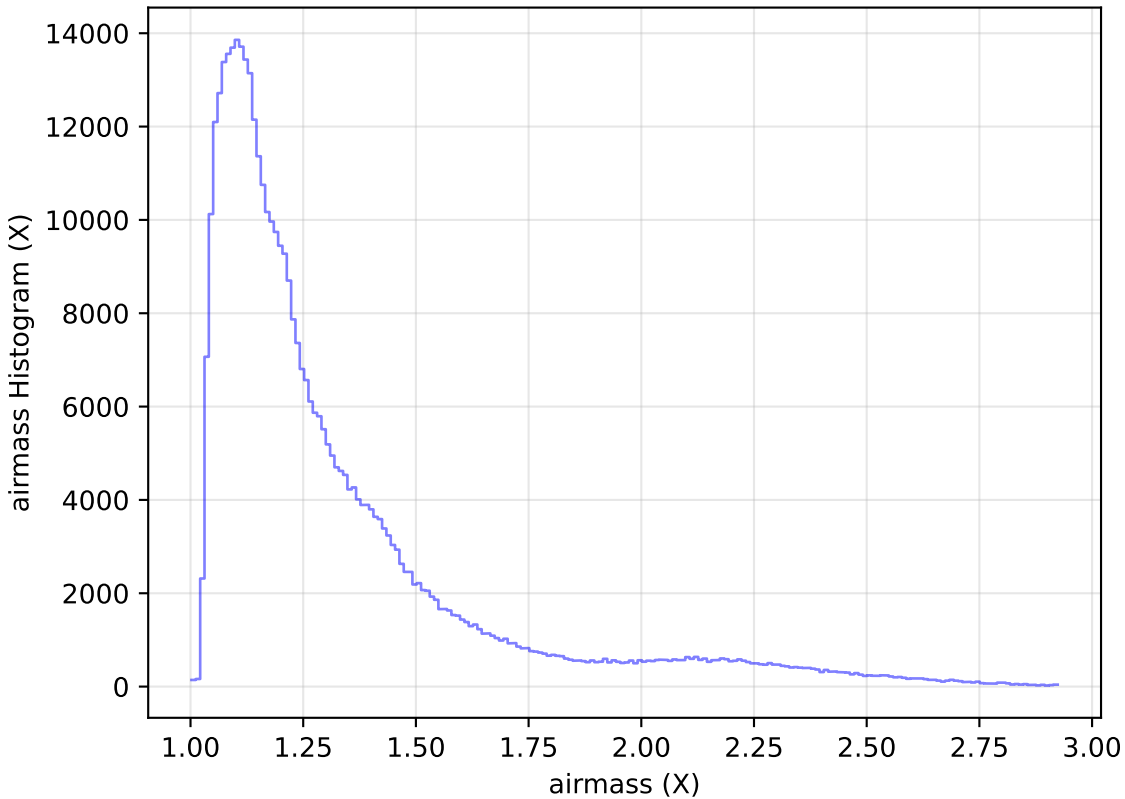
too_ignore_5_4v3.4_10yrs WFD z band: airmass Histogram
