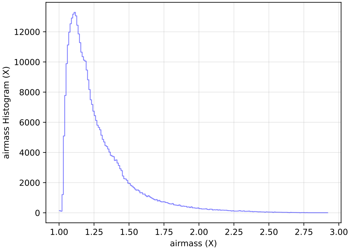
too_ignore_5_4v3.4_10yrs WFD y band: airmass Histogram
