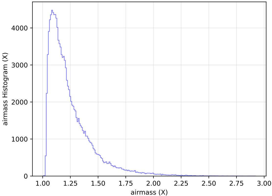
too_ignore_5_4v3.4_10yrs WFD u band: airmass Histogram
