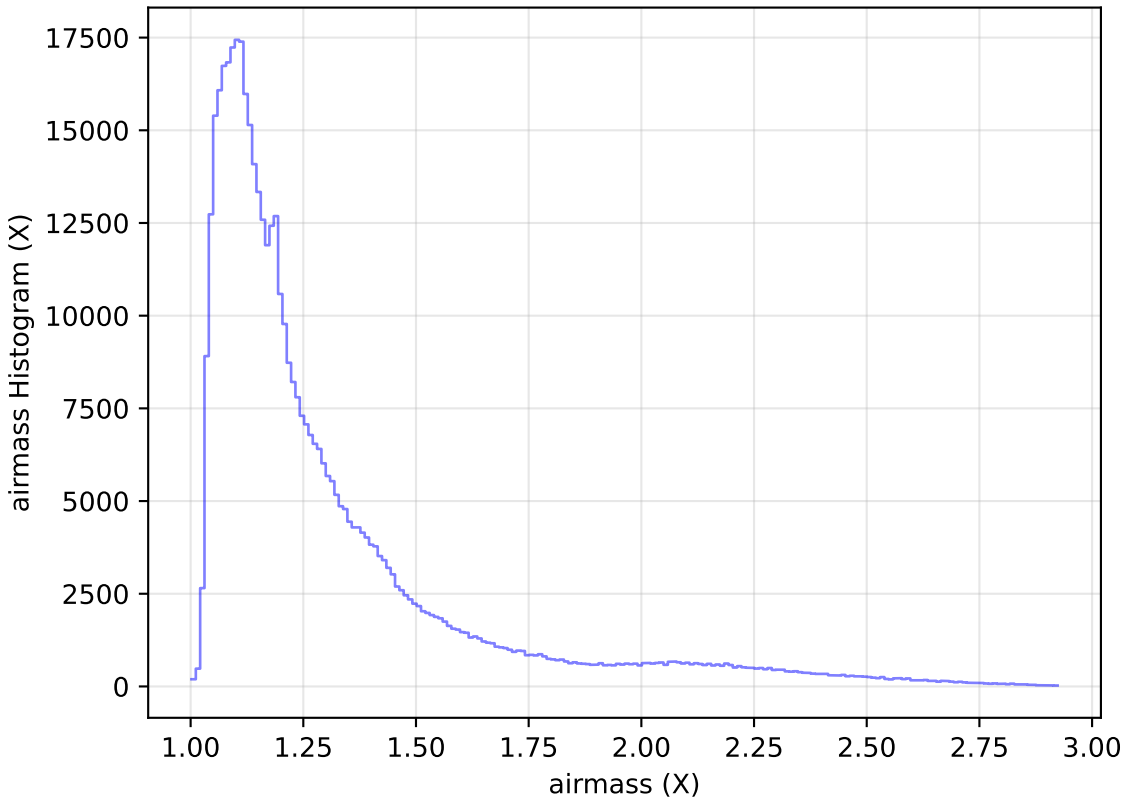
too_ignore_5_4v3.4_10yrs WFD i band: airmass Histogram
