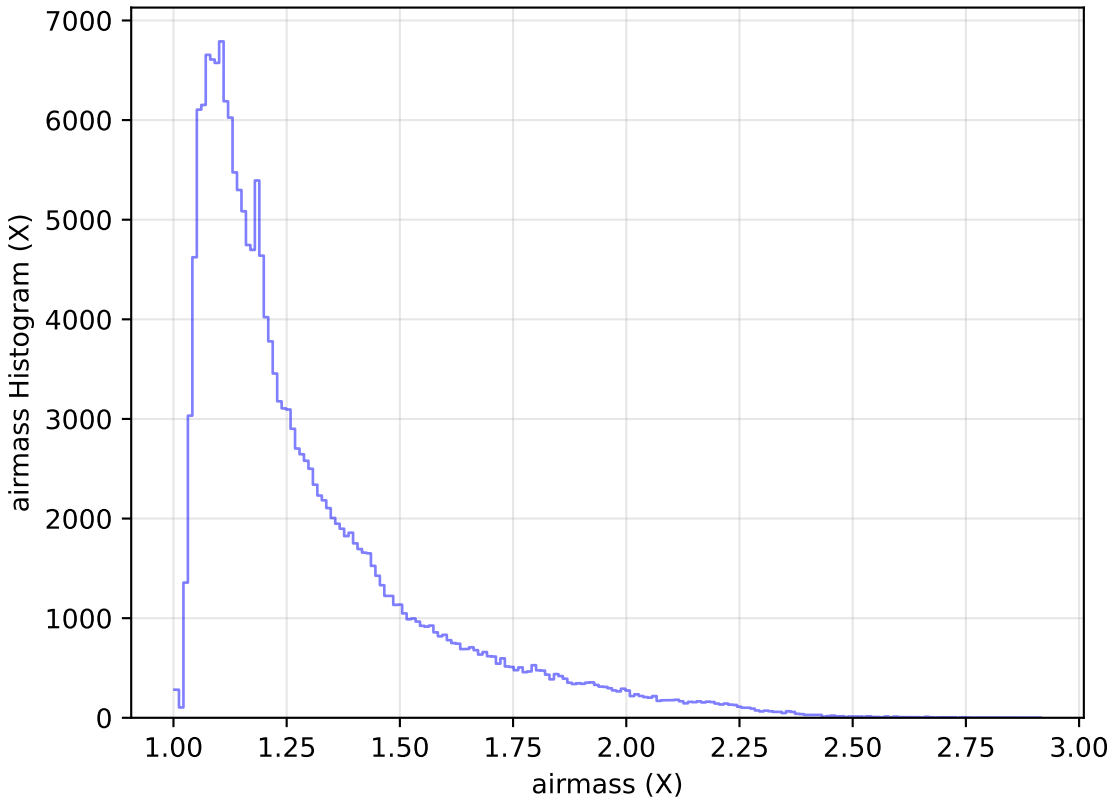
too_ignore_5_4v3.4_10yrs WFD g band: airmass Histogram
