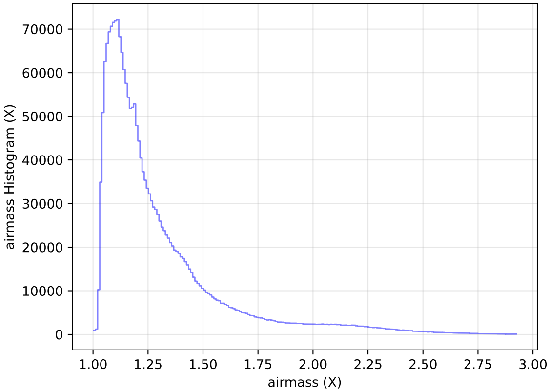
too_ignore_5_4v3.4_10yrs WFD all bands: airmass Histogram
