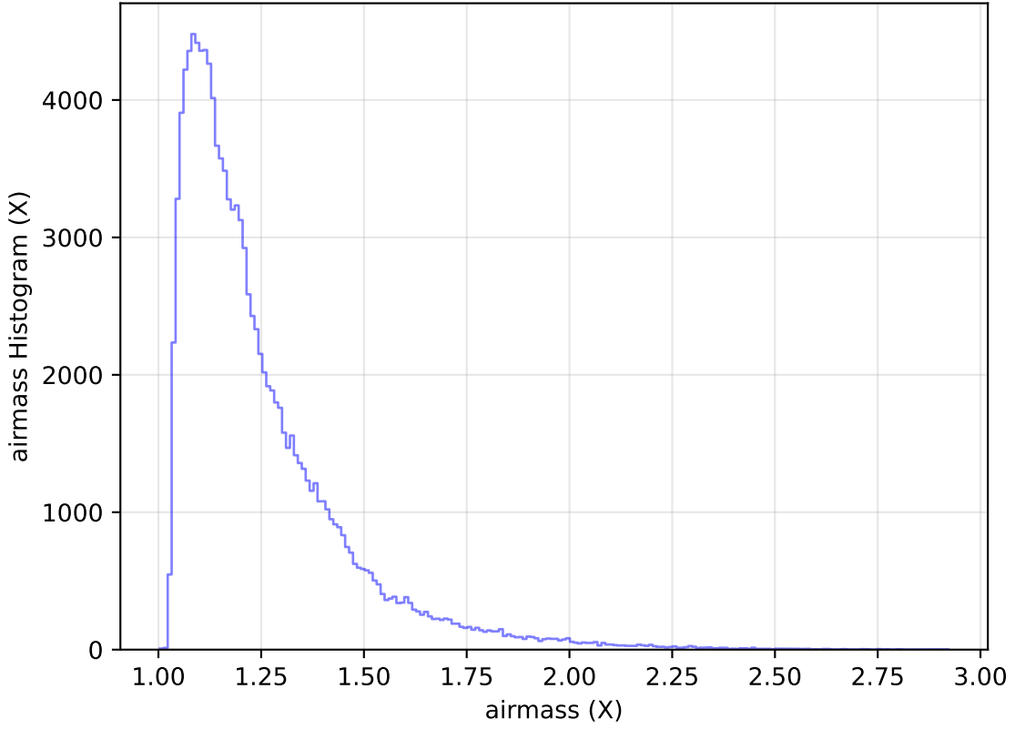
too_ignore_5_4v3.4_10yrs All sky u band: airmass Histogram
