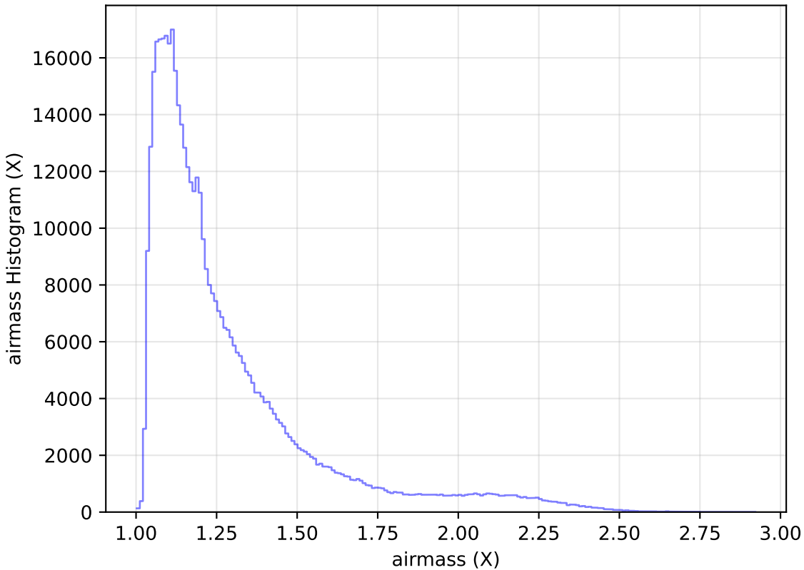
too_ignore_5_4v3.4_10yrs All sky r band: airmass Histogram
