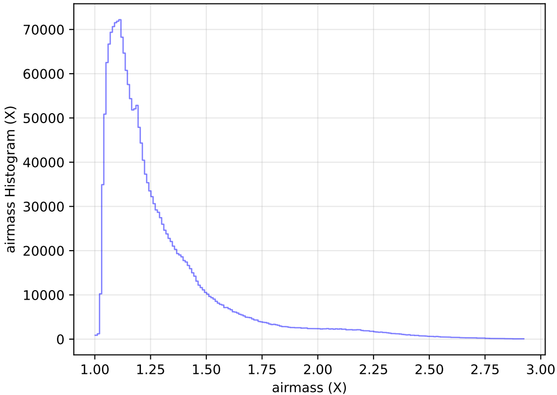
too_ignore_5_4v3.4_10yrs All sky all bands: airmass Histogram
