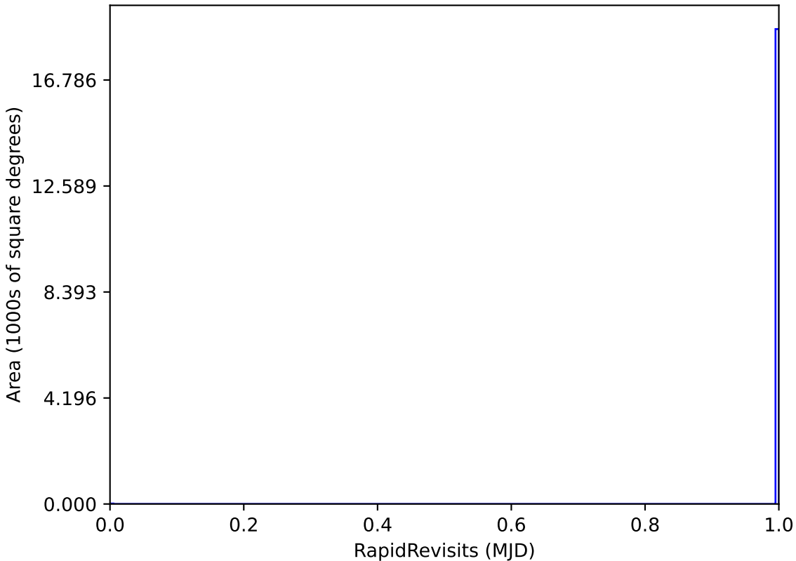
too_ignore_5_4v3.4_10yrs WFD: RapidRevisits
