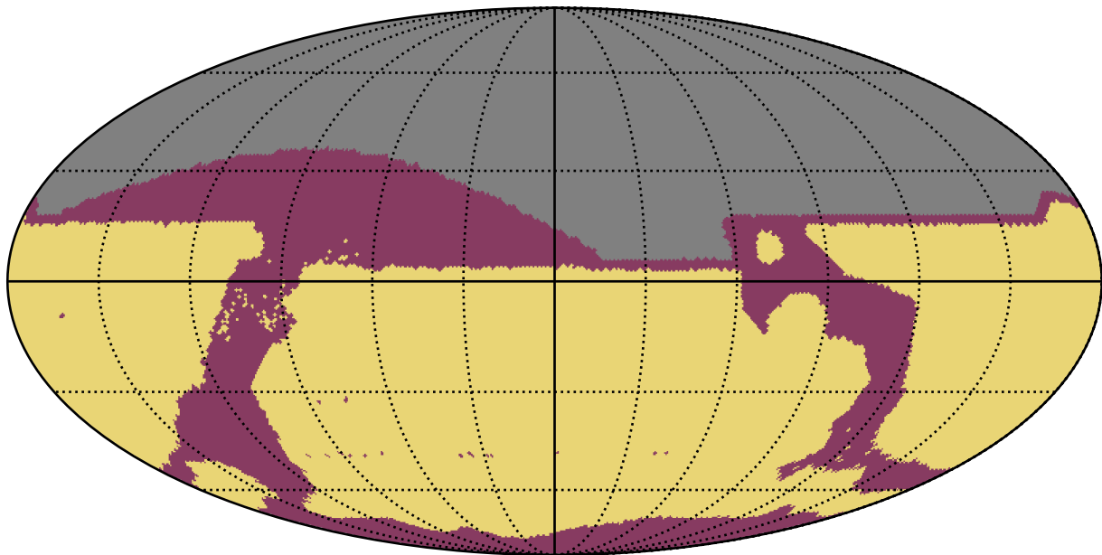
too_ignore_5_4v3.4_10yrs All sky: RapidRevisits
