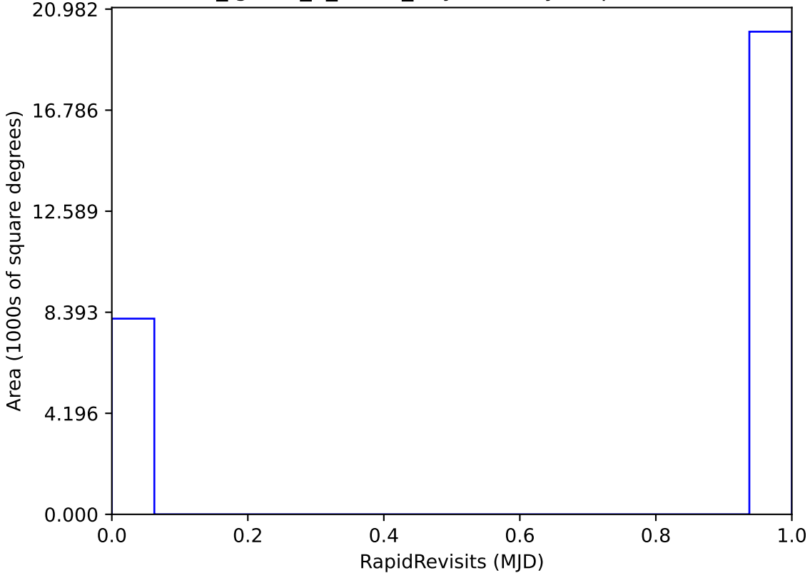
too_ignore_5_4v3.4_10yrs All sky: RapidRevisits
