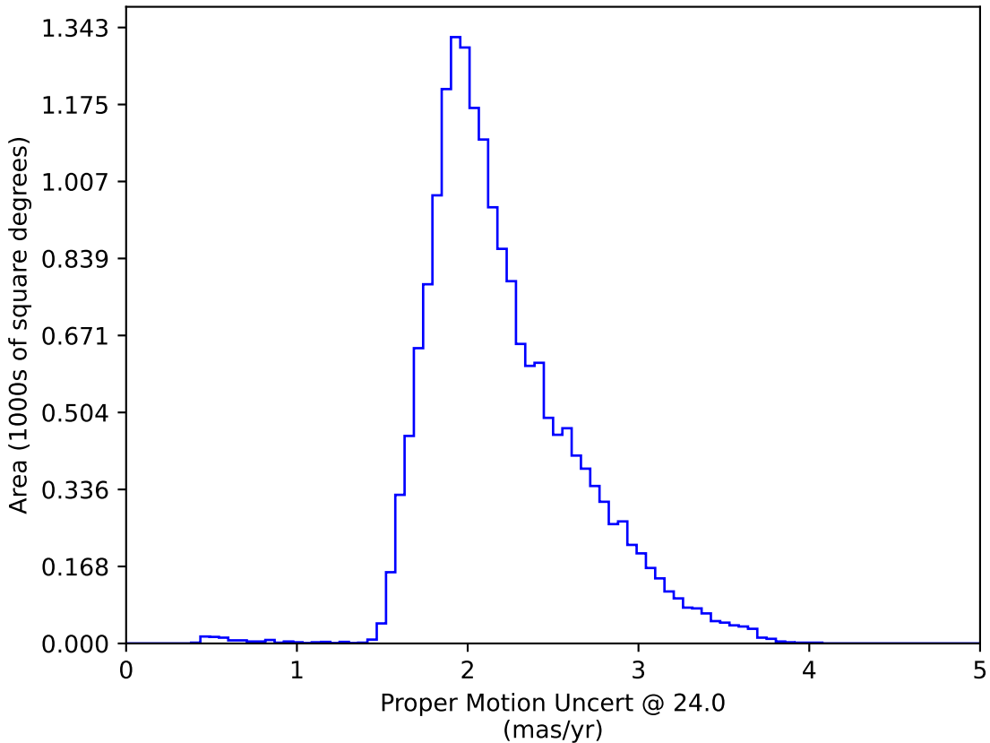
too_ignore_5_4v3.4_10yrs WFD: Proper Motion Uncert @ 24.0
