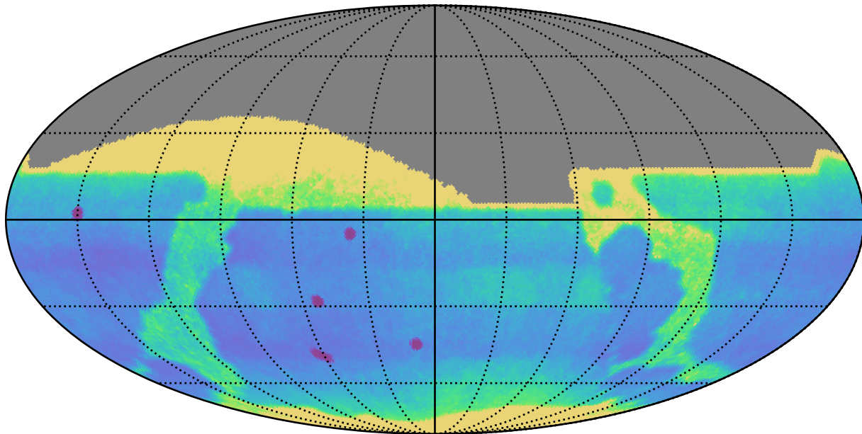
too_ignore_5_4v3.4_10yrs All sky: Proper Motion Uncert @ 24.0
