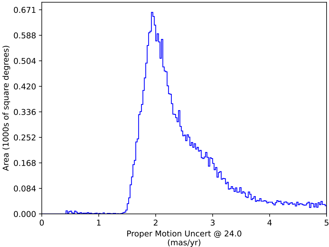
too_ignore_5_4v3.4_10yrs All sky: Proper Motion Uncert @ 24.0
