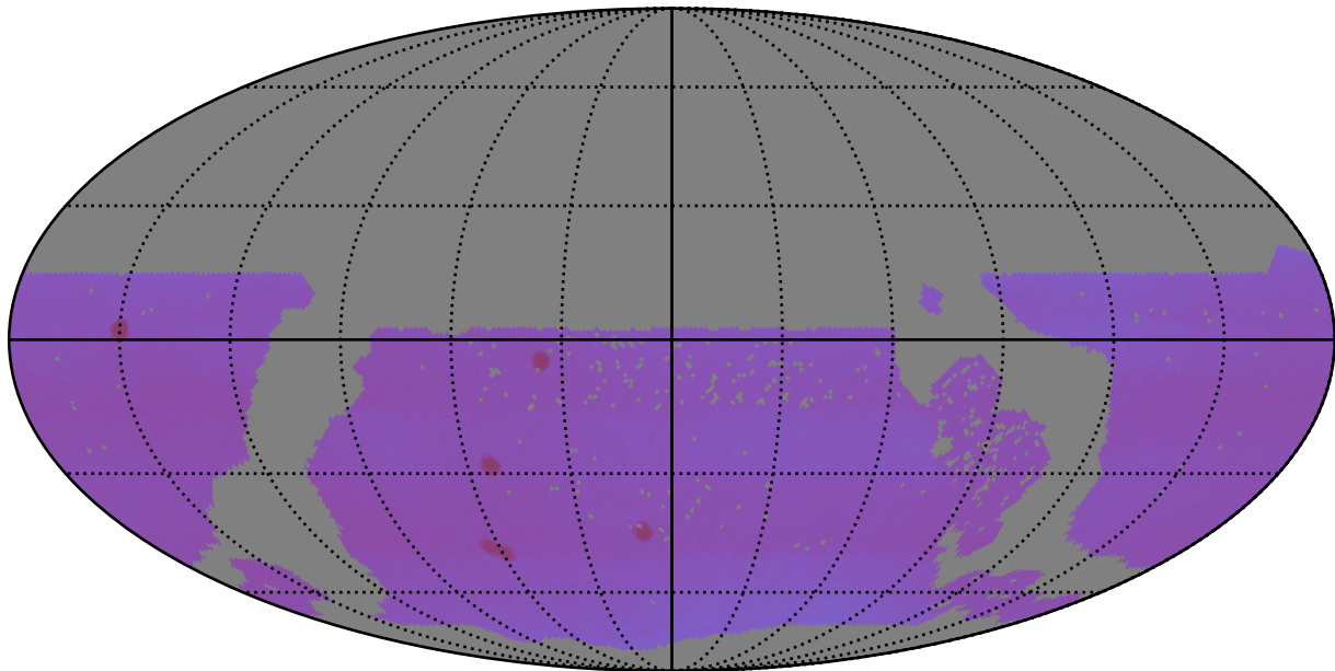
too_ignore_5_4v3.4_10yrs WFD: Proper Motion Uncert @ 20.5
