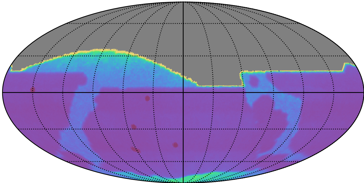
too_ignore_5_4v3.4_10yrs All sky: Proper Motion Uncert @ 20.5
