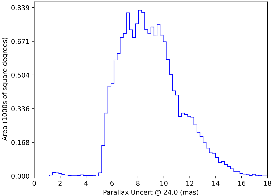
too_ignore_5_4v3.4_10yrs WFD: Parallax Uncert @ 24.0
