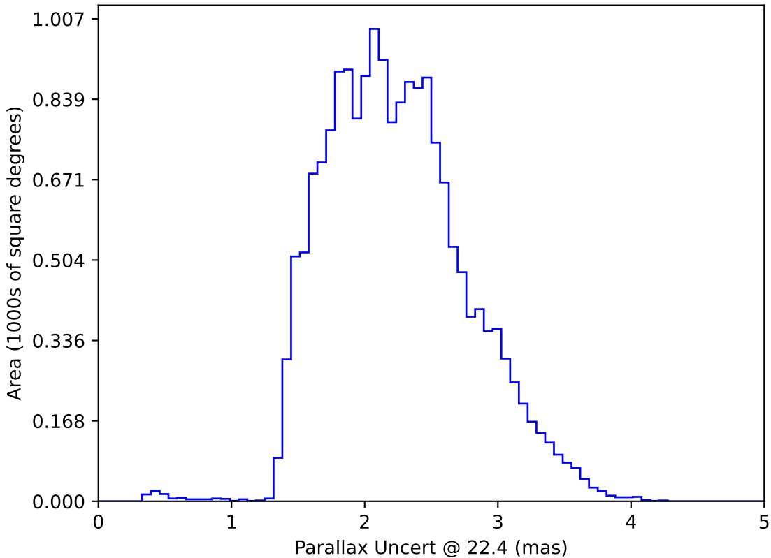
too_ignore_5_4v3.4_10yrs WFD: Parallax Uncert @ 22.4
