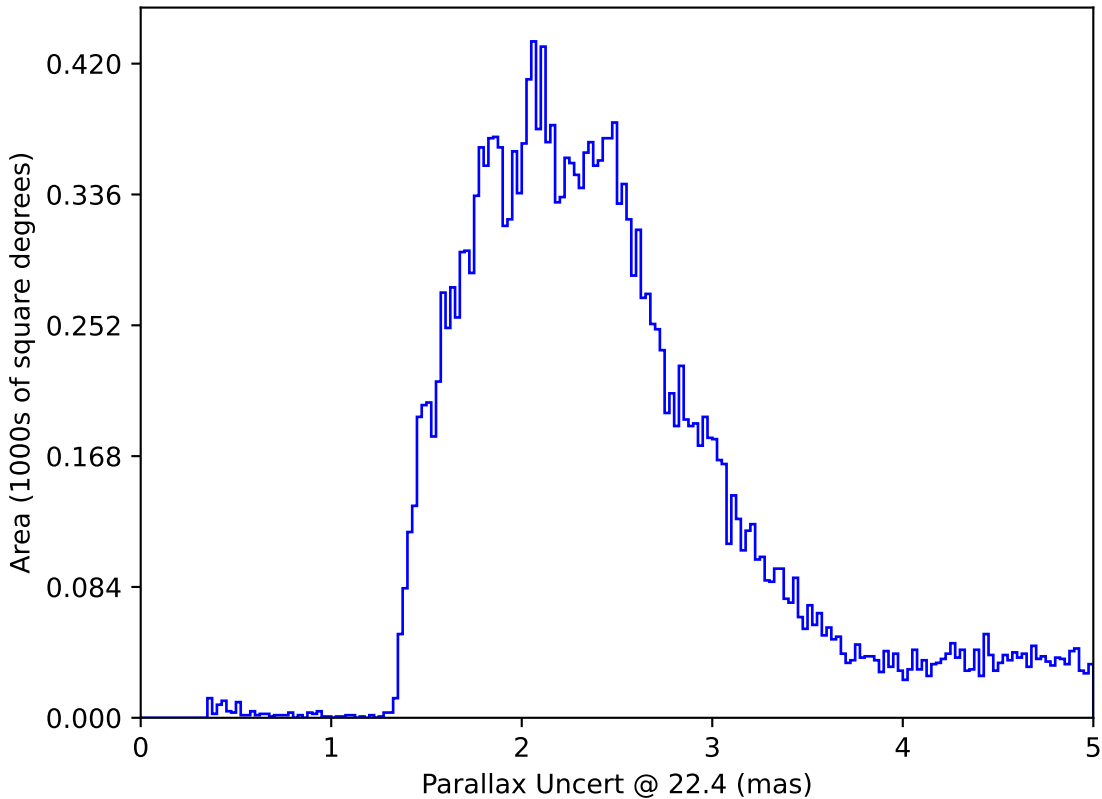
too_ignore_5_4v3.4_10yrs All sky: Parallax Uncert @ 22.4
