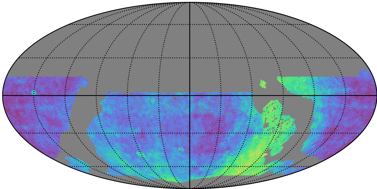
too_ignore_5_4v3.4_10yrs WFD: Parallax Coverage @ 24.0
