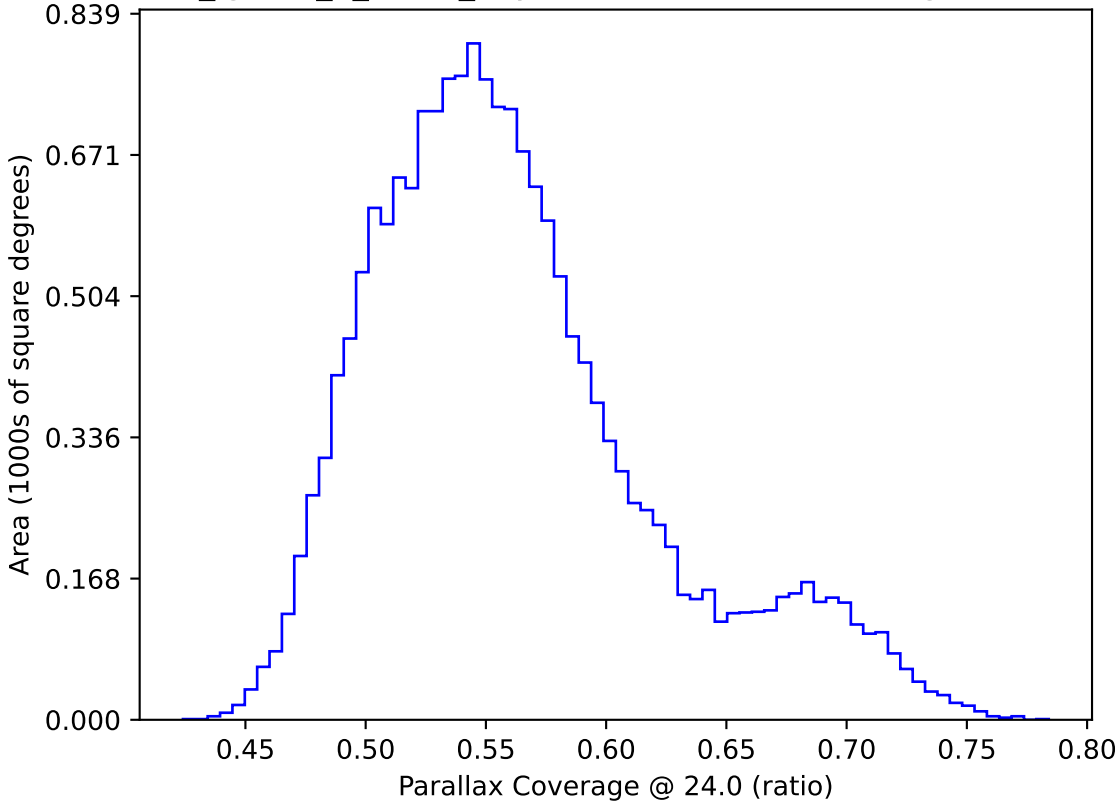
too_ignore_5_4v3.4_10yrs WFD: Parallax Coverage @ 24.0
