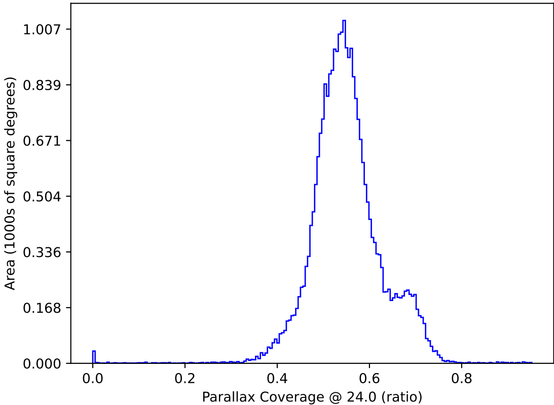
too_ignore_5_4v3.4_10yrs All sky: Parallax Coverage @ 24.0
