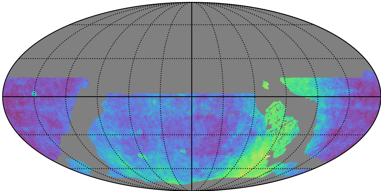
too_ignore_5_4v3.4_10yrs WFD: Parallax Coverage @ 22.4
