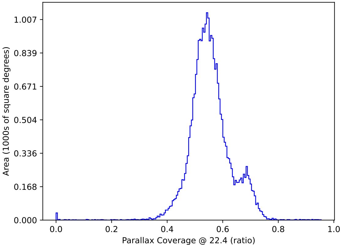
too_ignore_5_4v3.4_10yrs All sky: Parallax Coverage @ 22.4
