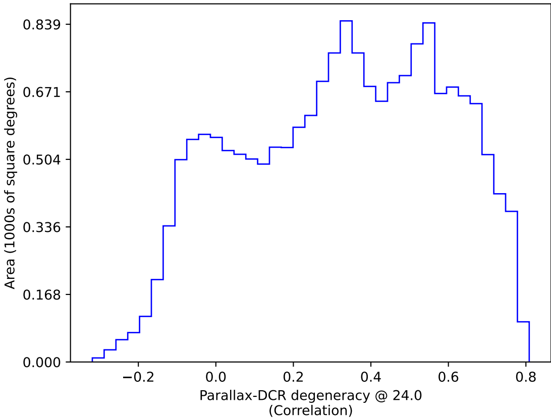
too_ignore_5_4v3.4_10yrs WFD: Parallax-DCR degeneracy @ 24.0
