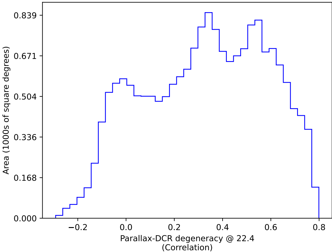
too_ignore_5_4v3.4_10yrs WFD: Parallax-DCR degeneracy @ 22.4
