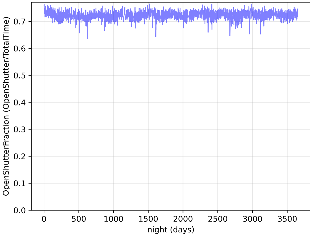
too_ignore_5_4v3.4_10yrs Per night: OpenShutterFraction
