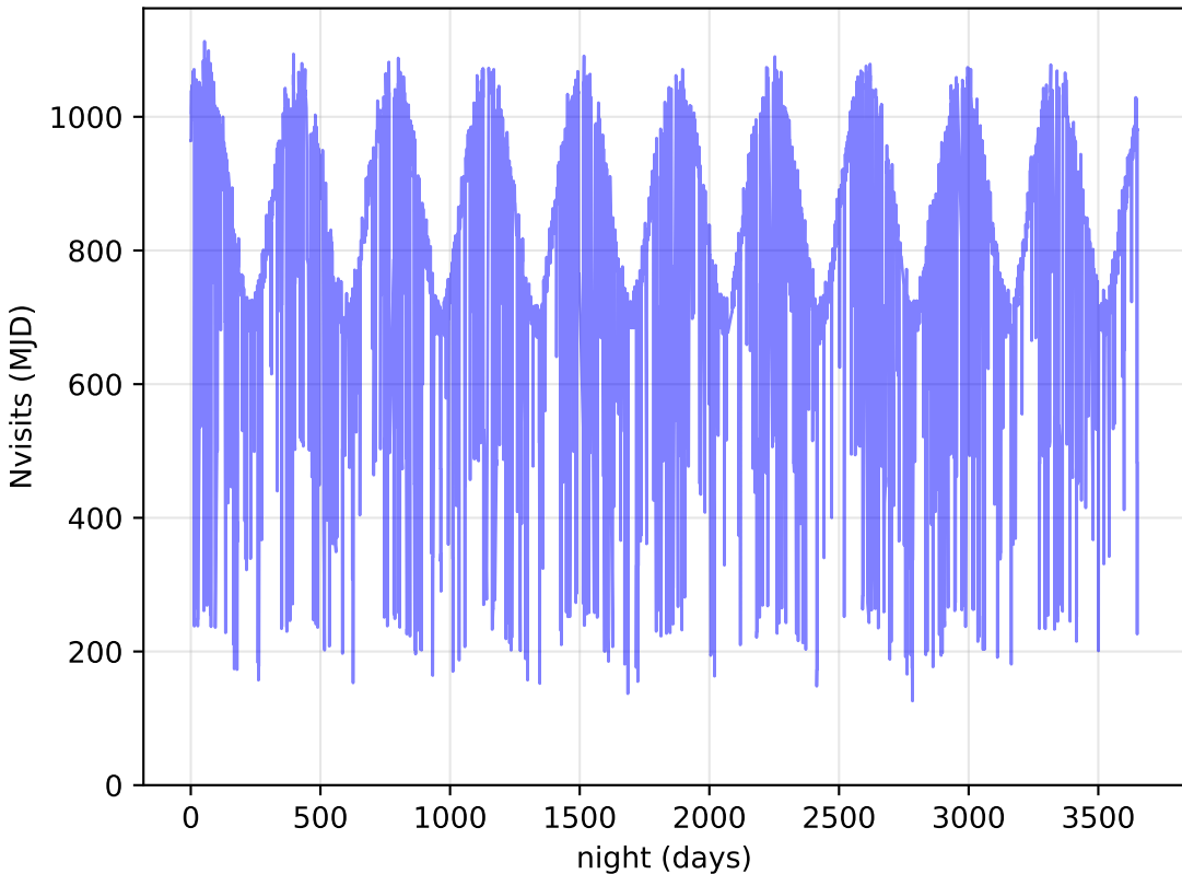
too_ignore_5_4v3.4_10yrs All visits: Nvisits
