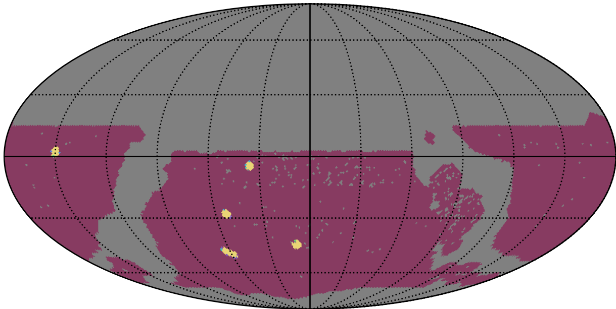
too_ignore_5_4v3.4_10yrs WFD: NumberOfQuickRevisits
