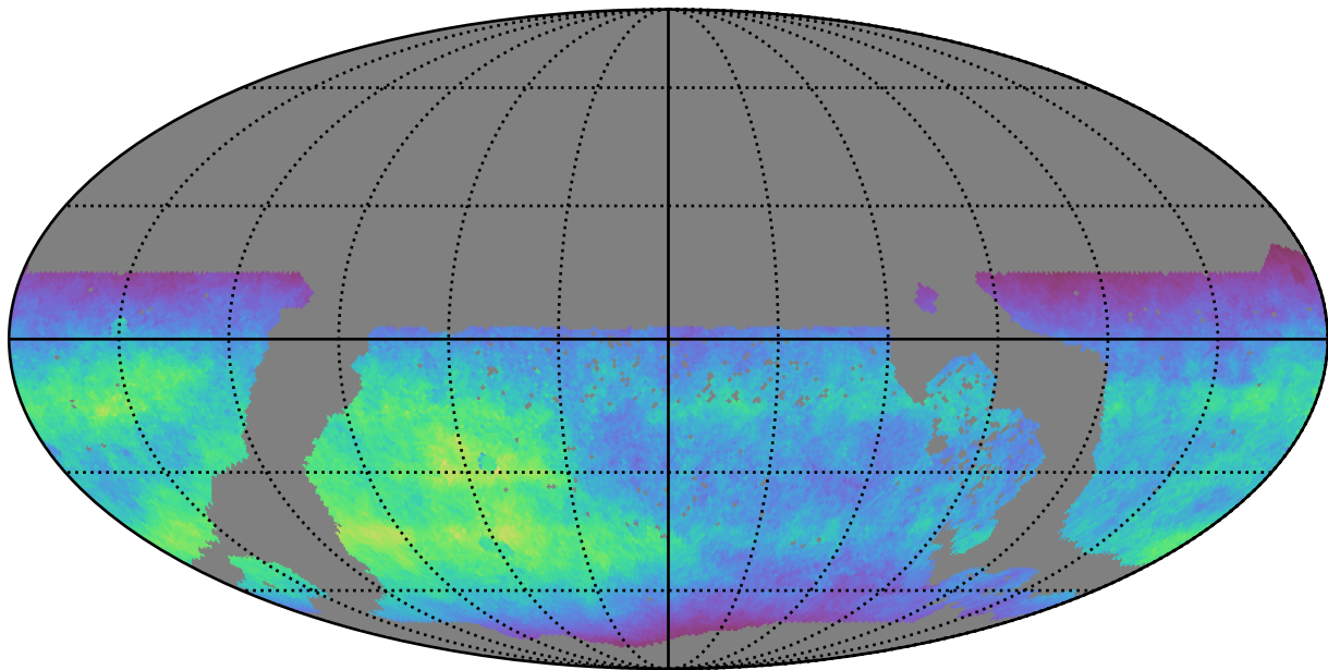
too_ignore_5_4v3.4_10yrs WFD z band: Normalized Teff
