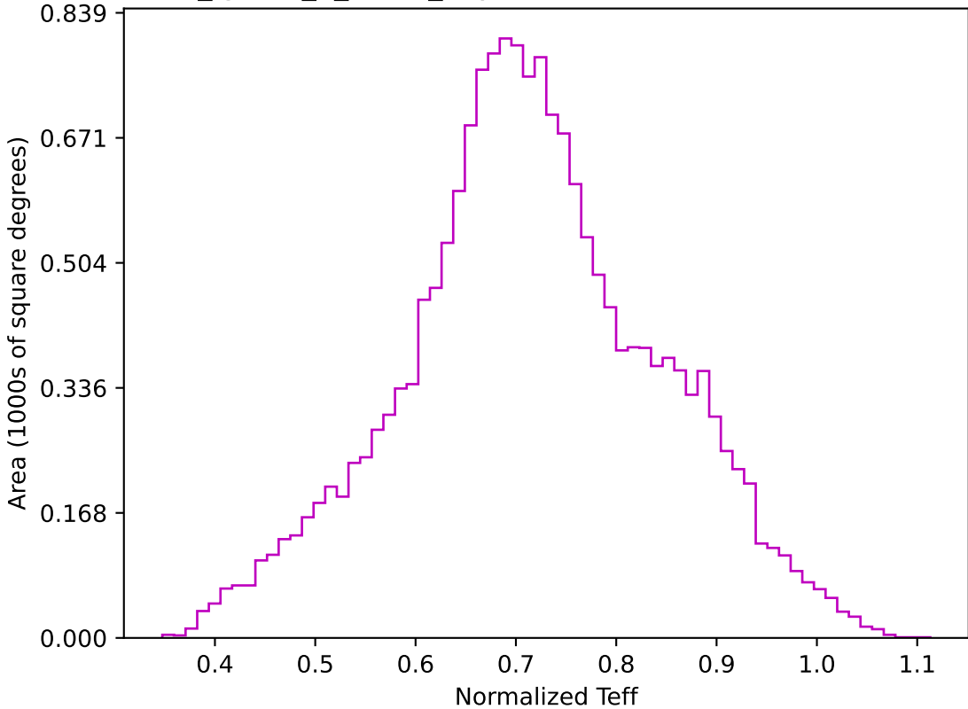
too_ignore_5_4v3.4_10yrs WFD z band: Normalized Teff
