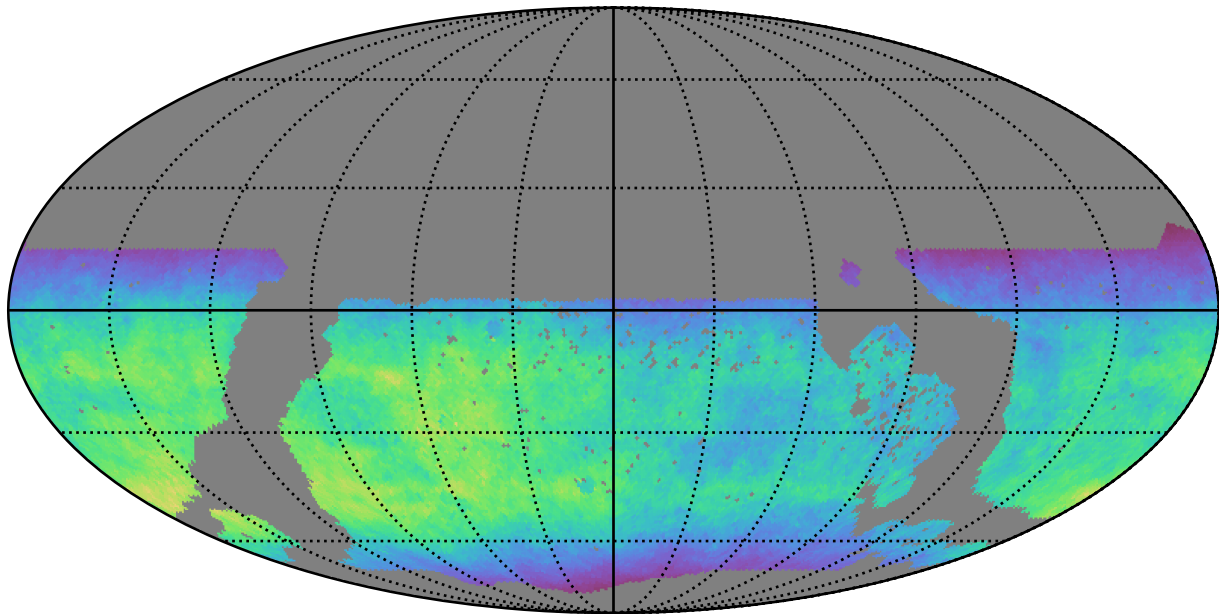
too_ignore_5_4v3.4_10yrs WFD y band: Normalized Teff
