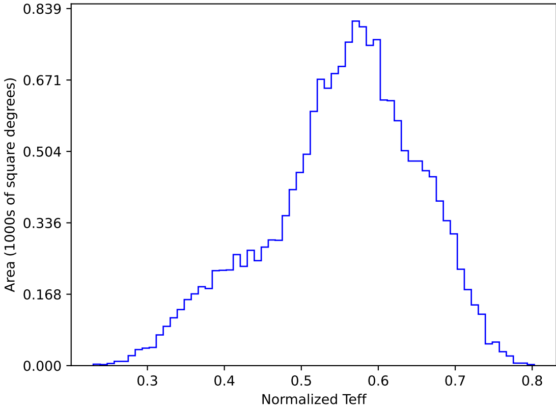
too_ignore_5_4v3.4_10yrs WFD y band: Normalized Teff
