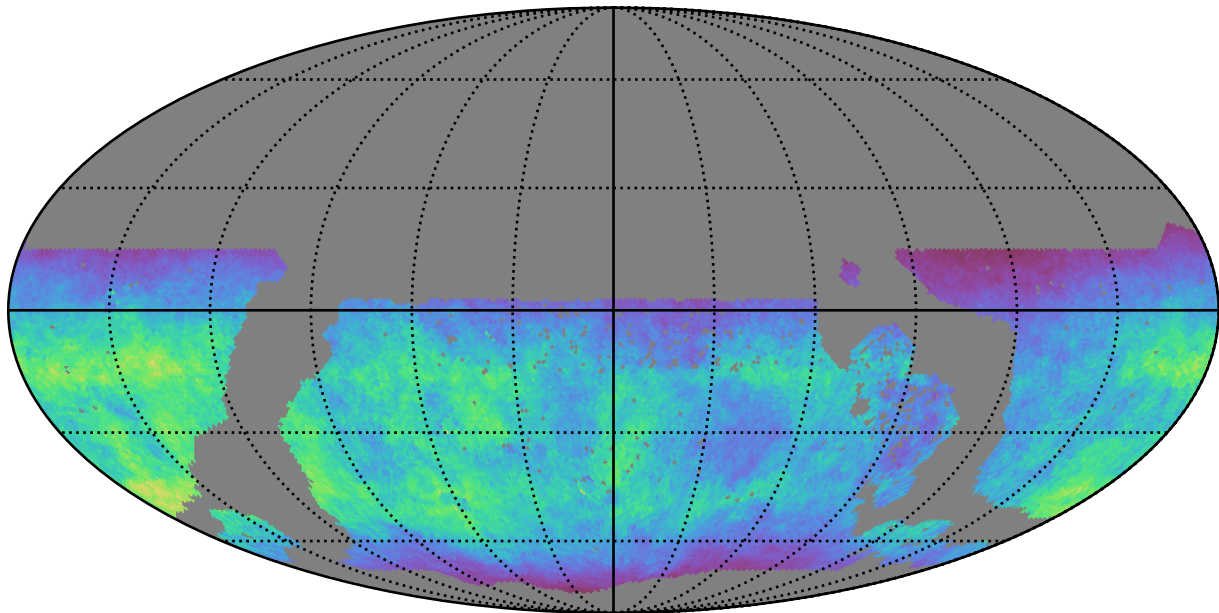
too_ignore_5_4v3.4_10yrs WFD u band: Normalized Teff
