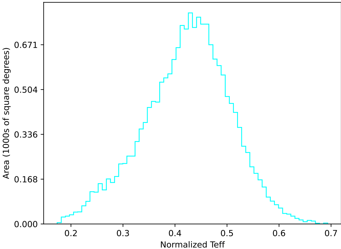
too_ignore_5_4v3.4_10yrs WFD u band: Normalized Teff
