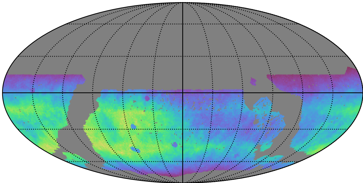
too_ignore_5_4v3.4_10yrs WFD r band: Normalized Teff
