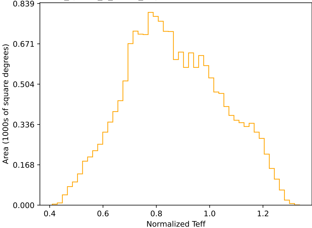
too_ignore_5_4v3.4_10yrs WFD r band: Normalized Teff
