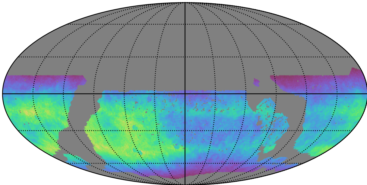
too_ignore_5_4v3.4_10yrs WFD i band: Normalized Teff
