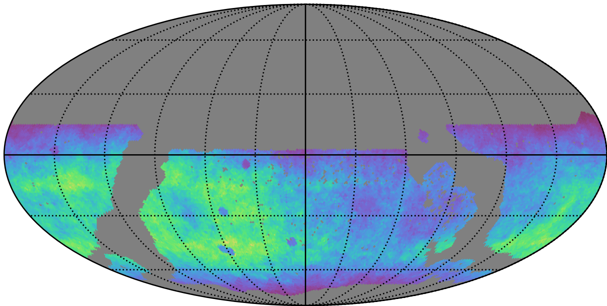
too_ignore_5_4v3.4_10yrs WFD g band: Normalized Teff
