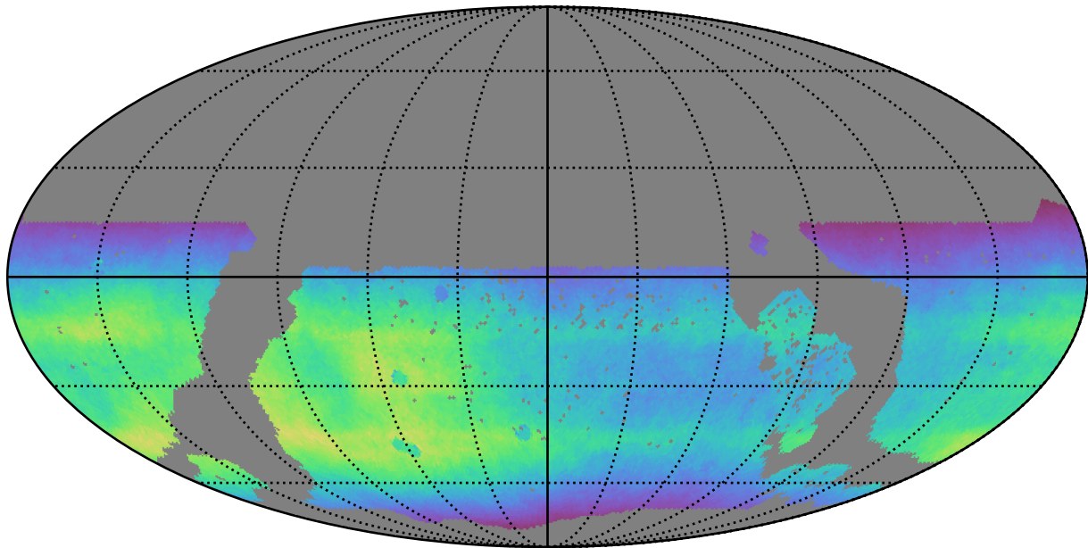
too_ignore_5_4v3.4_10yrs WFD all bands: Normalized Teff
