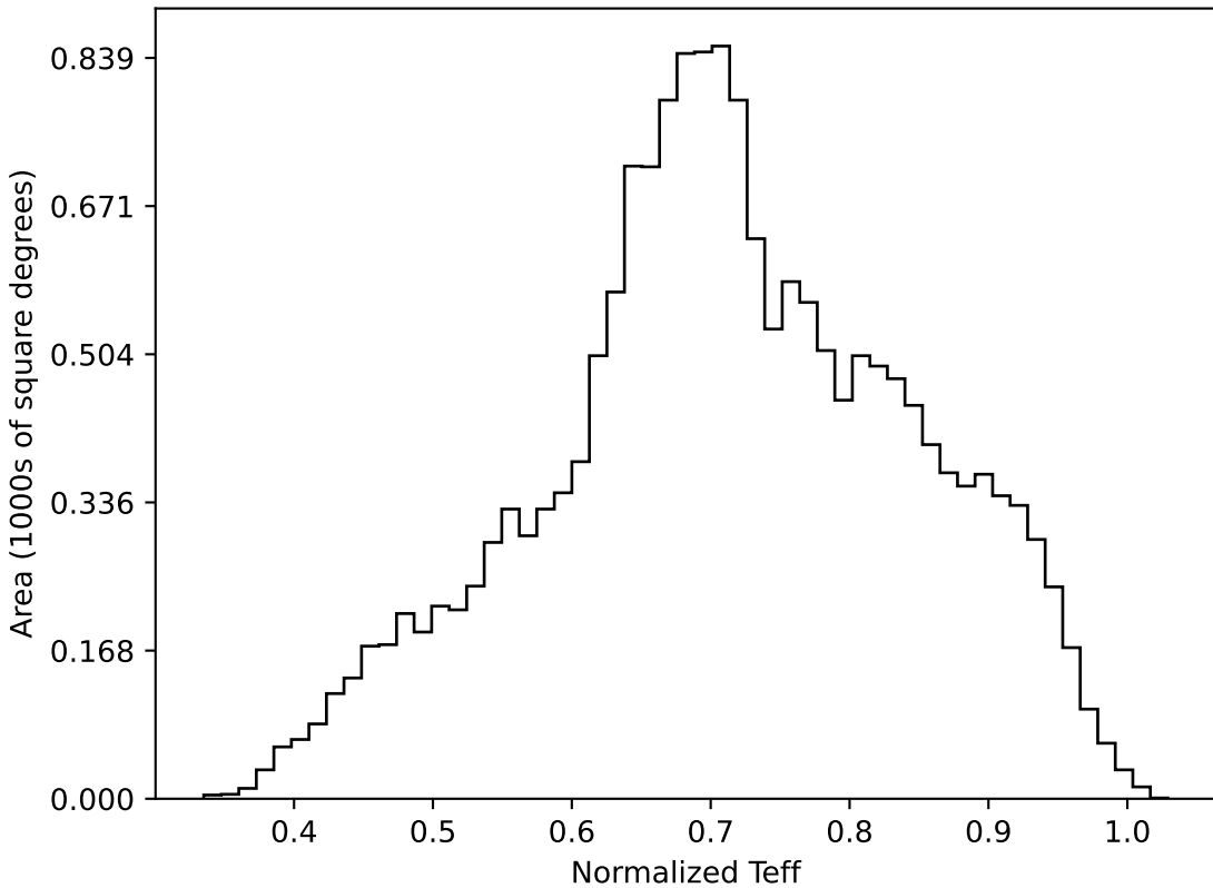
too_ignore_5_4v3.4_10yrs WFD all bands: Normalized Teff
