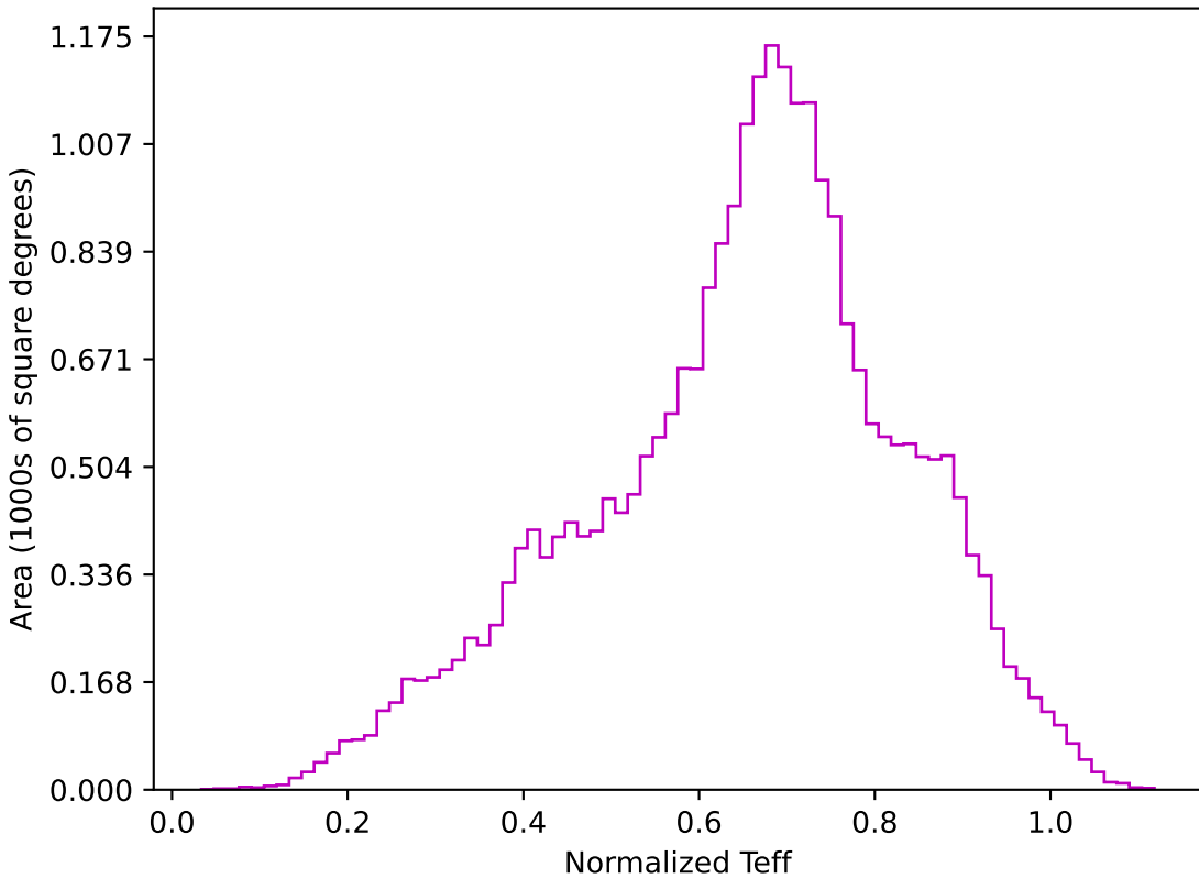
too_ignore_5_4v3.4_10yrs All sky z band: Normalized Teff
