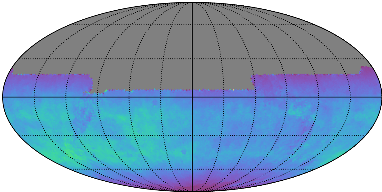
too_ignore_5_4v3.4_10yrs All sky y band: Normalized Teff
