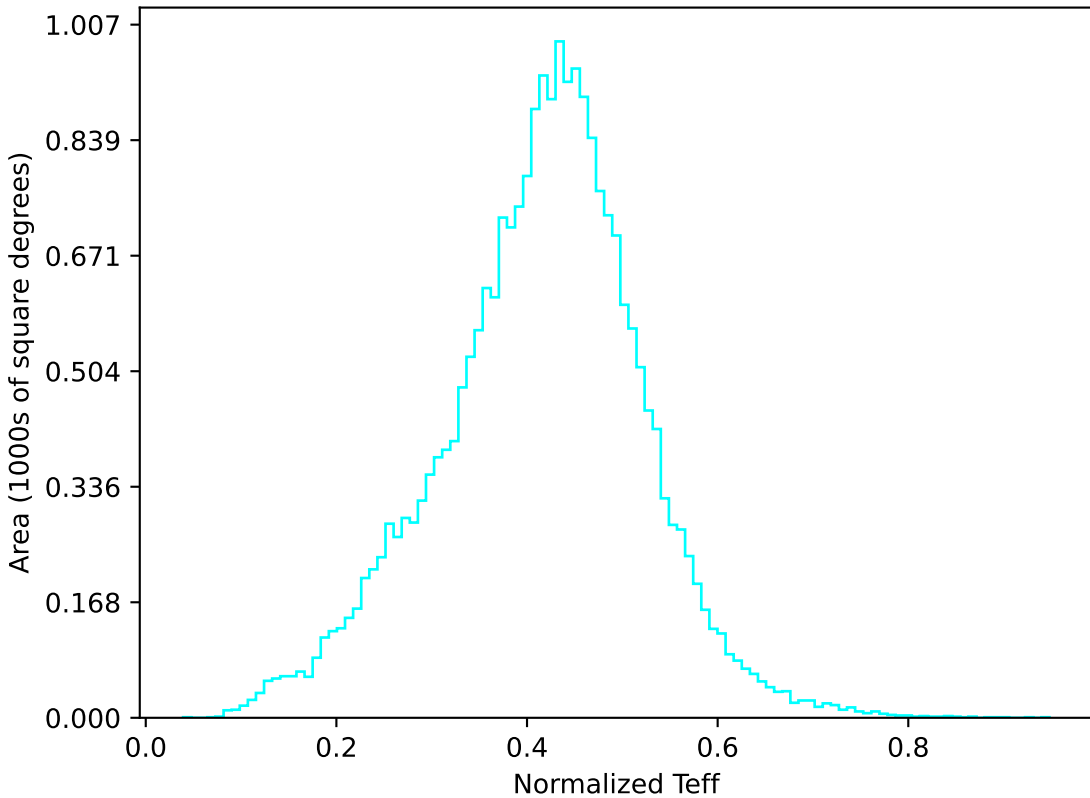
too_ignore_5_4v3.4_10yrs All sky u band: Normalized Teff
