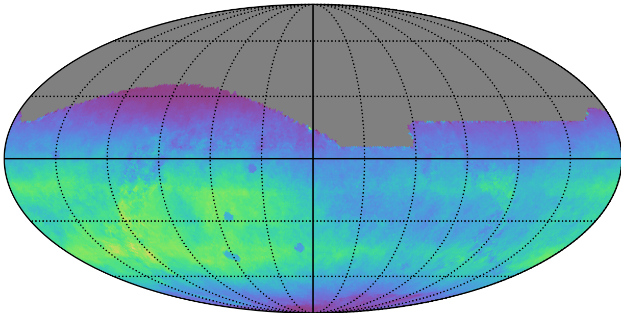
too_ignore_5_4v3.4_10yrs All sky r band: Normalized Teff
