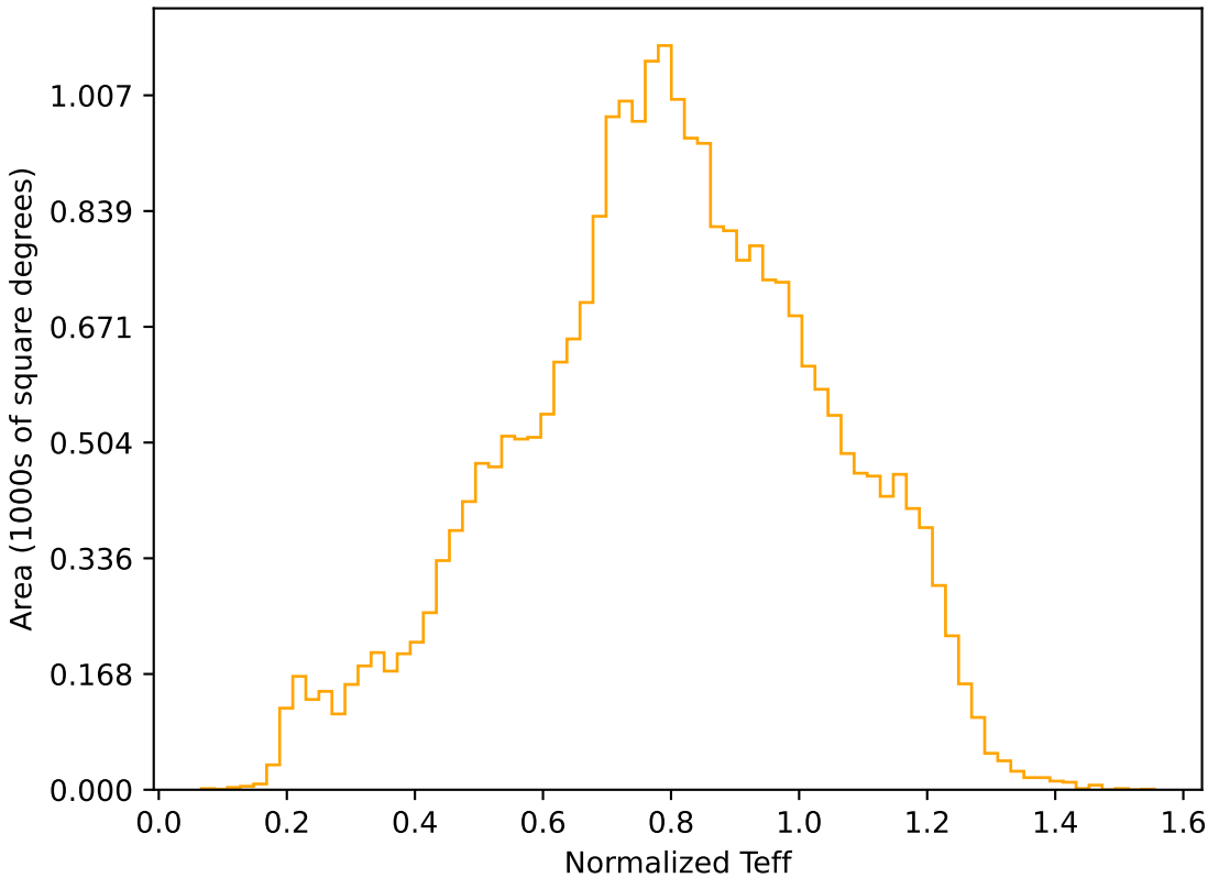
too_ignore_5_4v3.4_10yrs All sky r band: Normalized Teff
