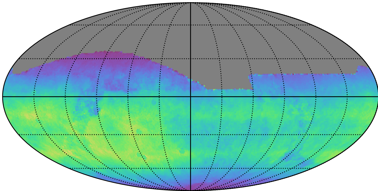
too_ignore_5_4v3.4_10yrs All sky i band: Normalized Teff
