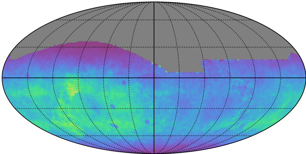
too_ignore_5_4v3.4_10yrs All sky g band: Normalized Teff
